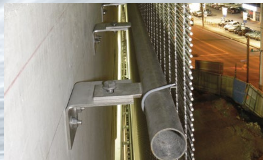
Intermediate mounting: round tube and wire connectors.
