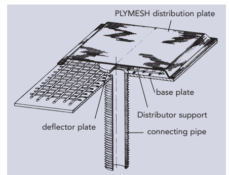
Configuration of a PLYMESH aeration pad
