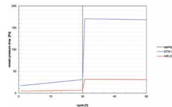
Purging properties according to VDI 3926.
