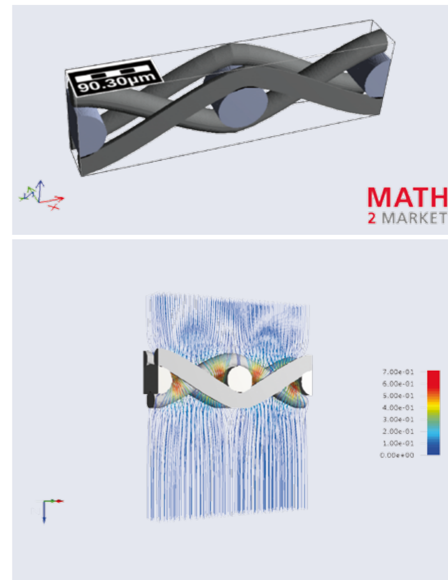
The cloth structure of the MINIMESH® S metal filter cloth is flow-optimized.
